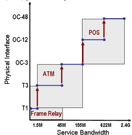
Figure 1: Service Bandwidth per TDM interface
