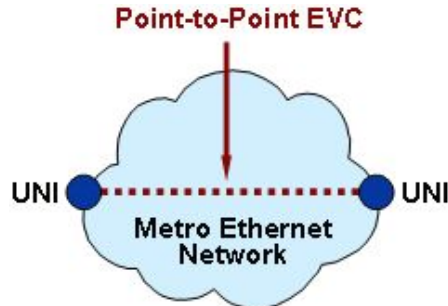
Figure 3: E-Line Service type using Point-to-Point EVC
