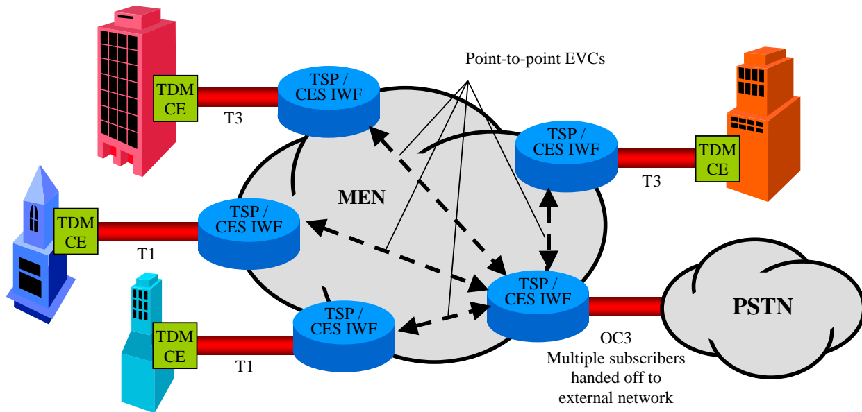
Figure 6: Possible TDM Handoff Configurations
