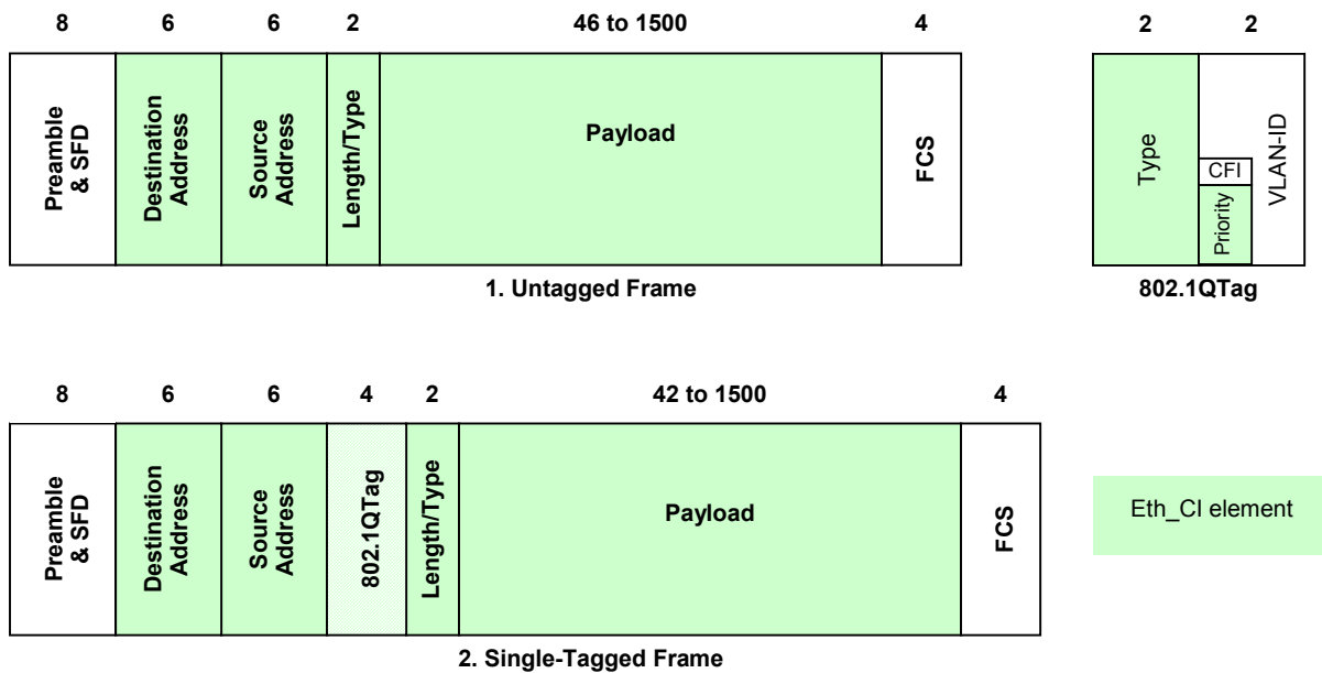
Figure 2: ETH Layer Characteristic Information (ETH_CI)
