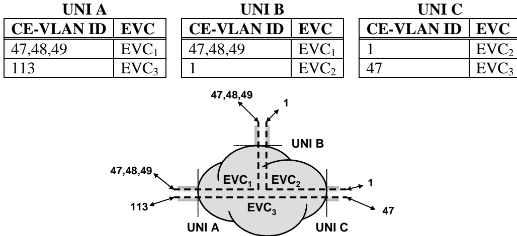
Figure 9 – Example of Bundling
