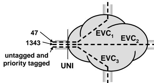
Figure 7 – Example of a CE-VLAN ID/EVC Map
