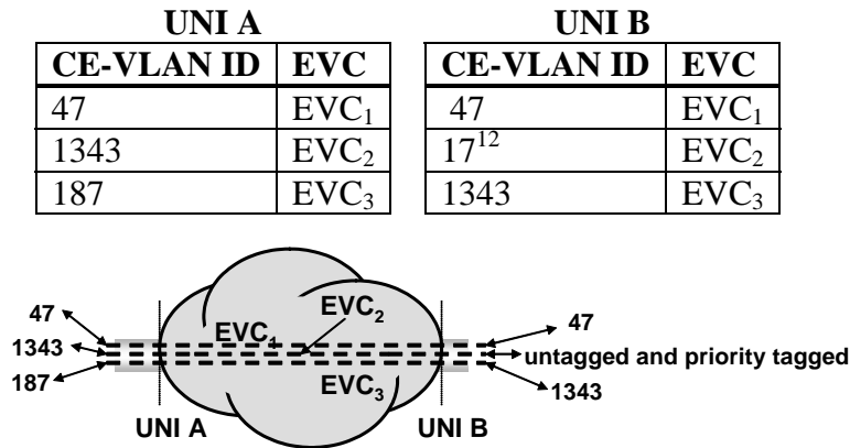
Figure 8 – Example of CE-VLAN ID/EVC Maps at Two UNIs
